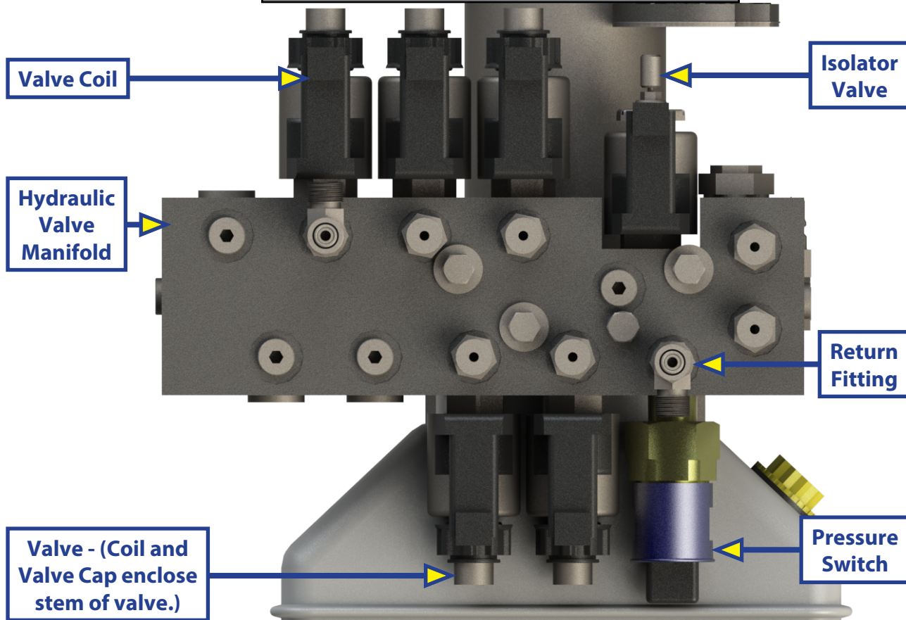
Fig. 11 - 4 Point Leveling +1 Slideout Manifold
